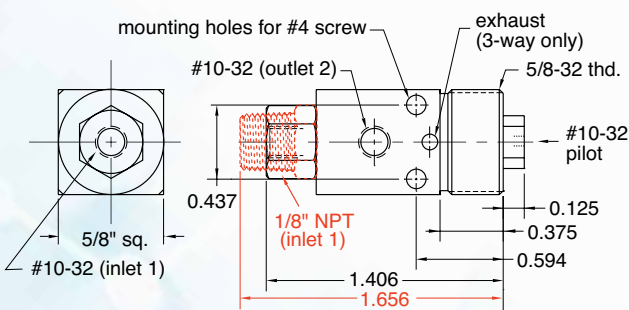
PAV-2P shown
