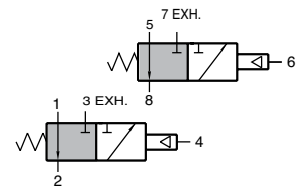
Normally-Open Double
