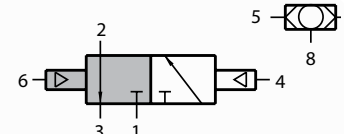
Normally-Closed shown
