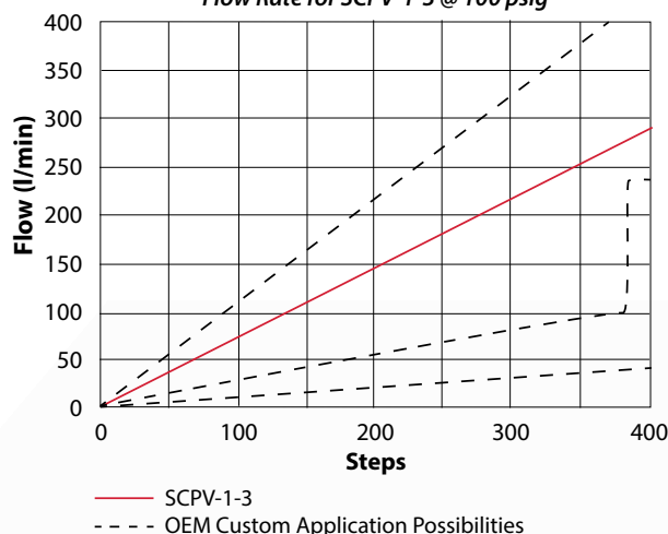
Characteristic Curve
